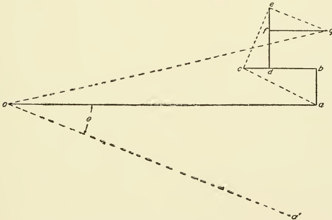
Fig. 27. Vector Diagram of Quantities Involved in Single-Phase
